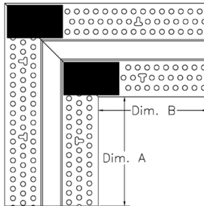
"L" Intersection
